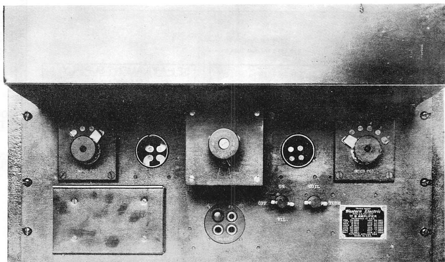
No. 17-B AMPLIFIER FRONT VIEW - COVER IN PLACE
