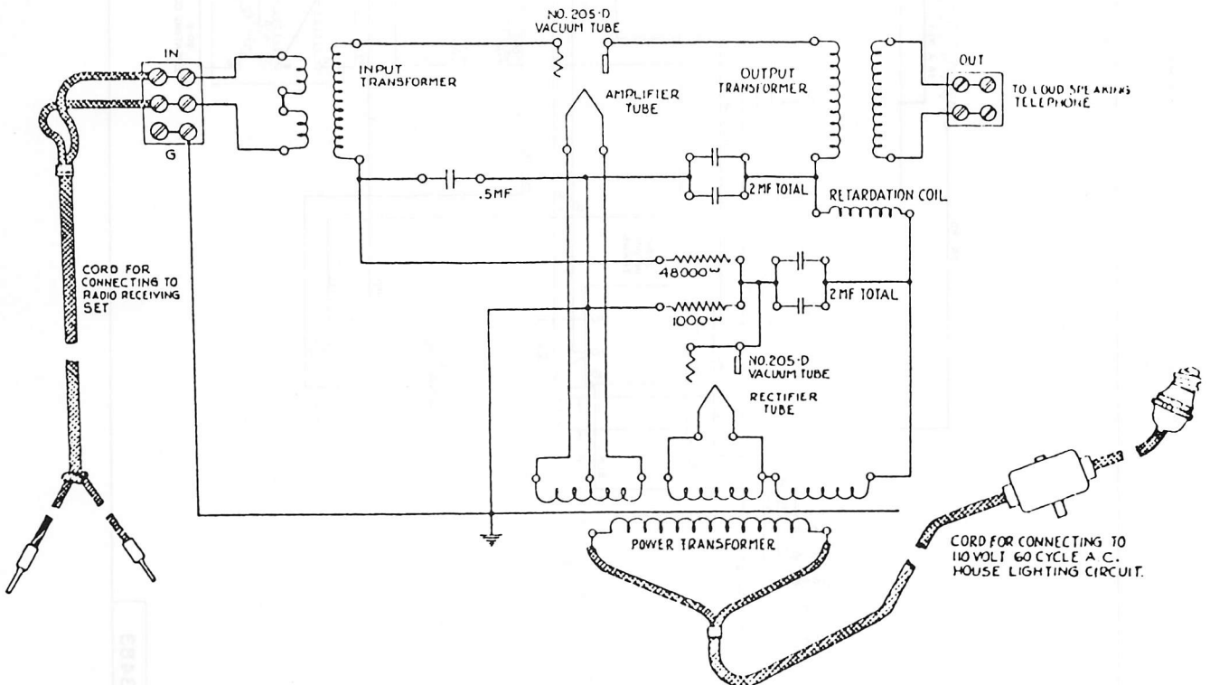
CIRCUIT DIAGRAM
